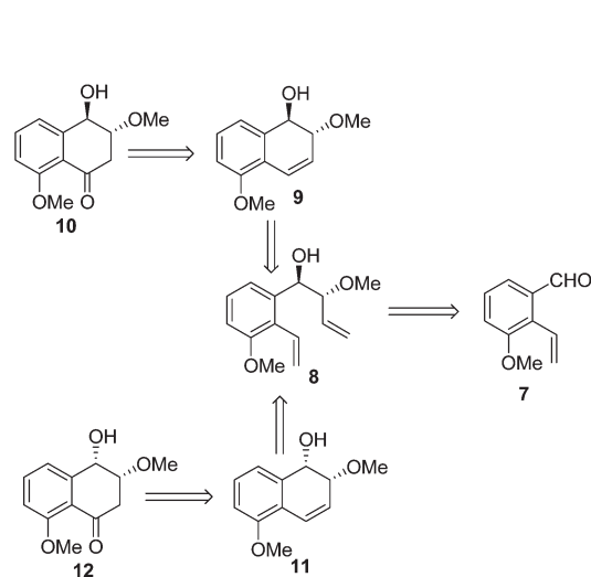
Fig. 1 Retrosynthetic analysis.
